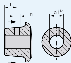
hub thread
