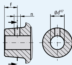
hub thread
