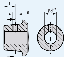
hub thread
