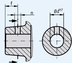
hub thread
